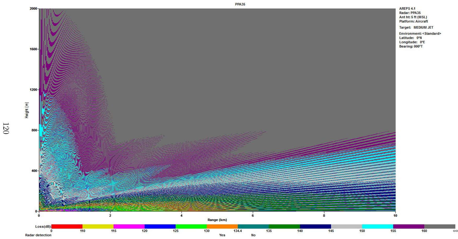
Figure 59. 35 GHz AREPS Propagation Loss for Surface-to-Air Scenario in Standard Atmosphere
