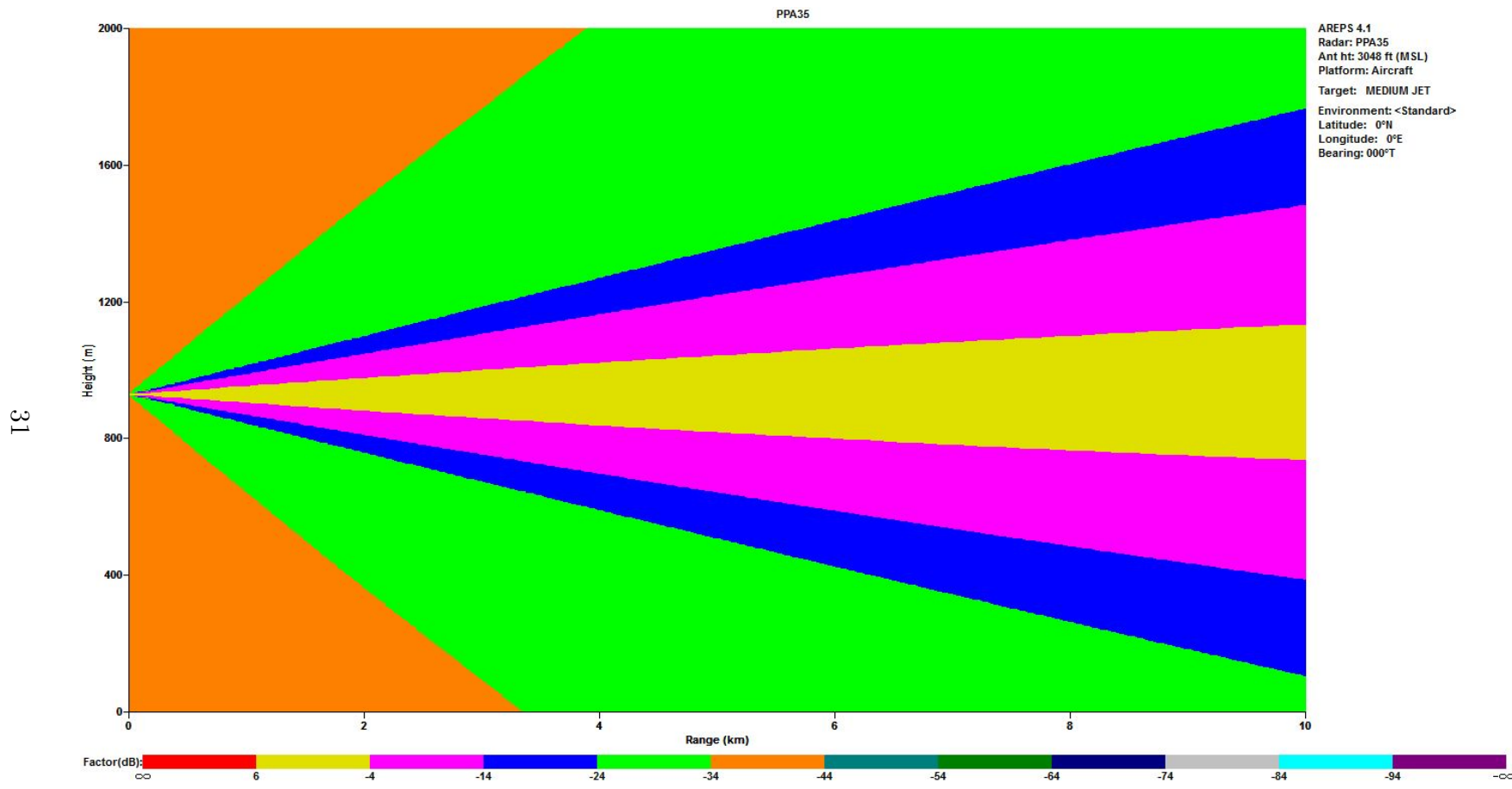
Figure 10. Example of AREPS Propagation Factor Plot
