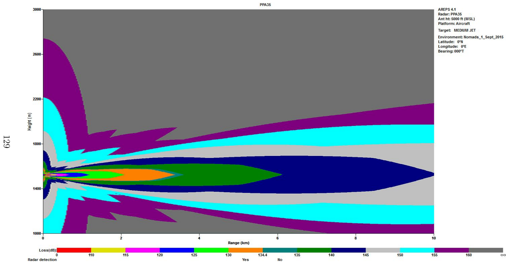
Figure 66. 35 GHz AREPS Propagation Loss for Air-to-Surface Scenario in NOMADS Atmosphere at 5,000 Feet
