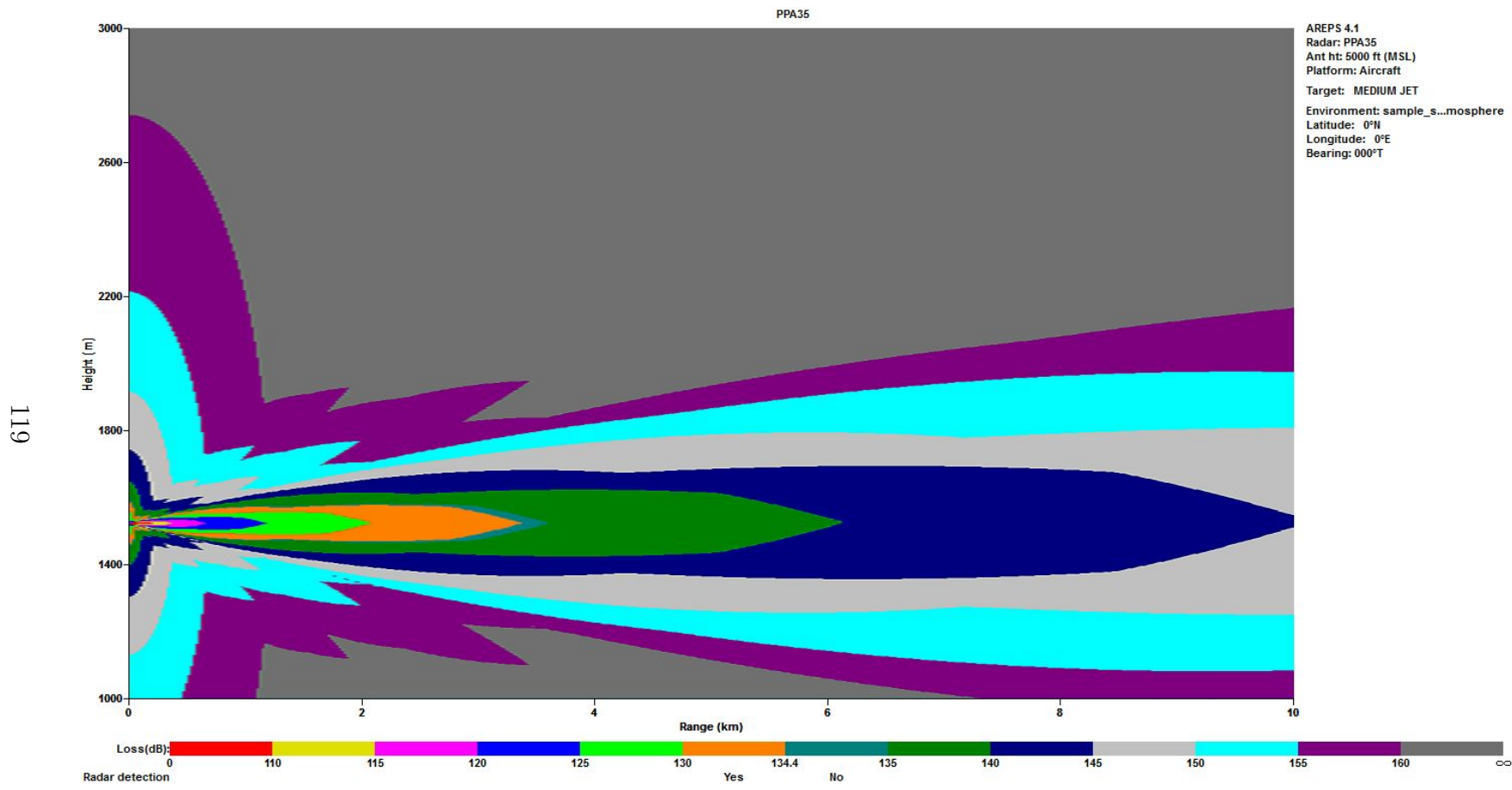
Figure 58. 35 GHz AREPS Propagation Loss for Air-to-Surface Scenario in Standard Atmosphere at 5,000 Feet
